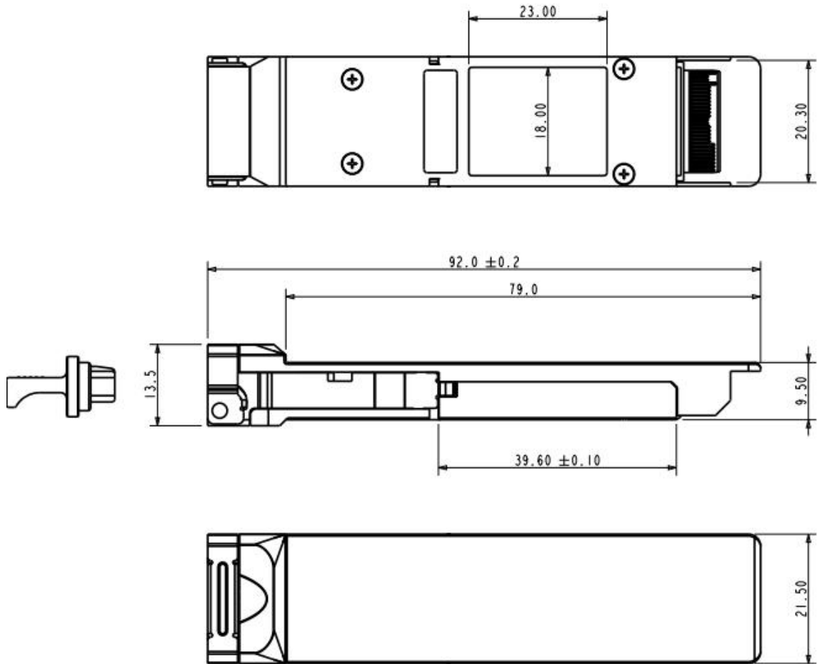
Figure 6.Mechanical Outline
