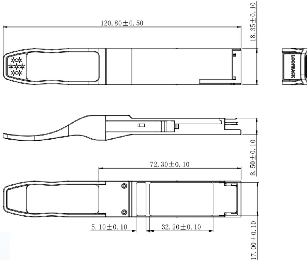
Figure 8. Mechanical Specifications
