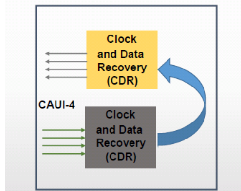
Figure 1. Module Block Diagram
