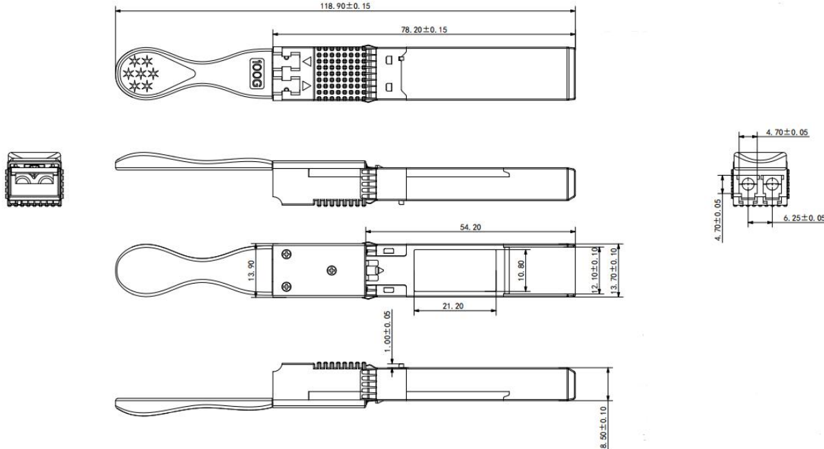
Figure 8. Mechanical Specifications
