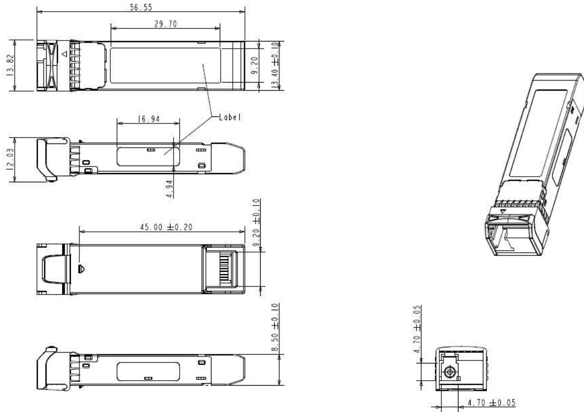
Figure 3. Mechanical Specifications
