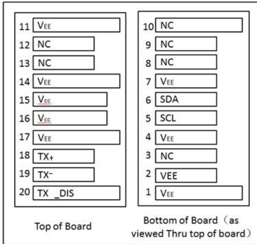
Figure 2. Electrical Pin-out Details
