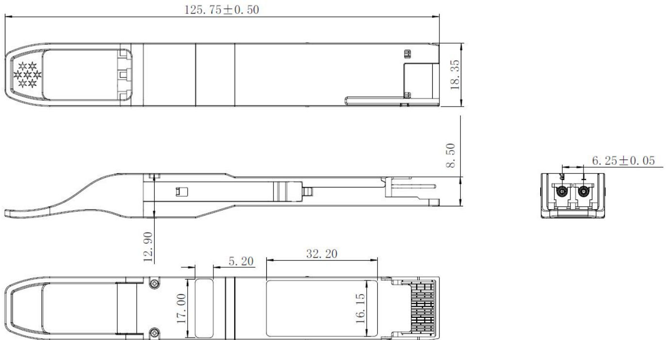
Figure6. Mechanical Specifications
