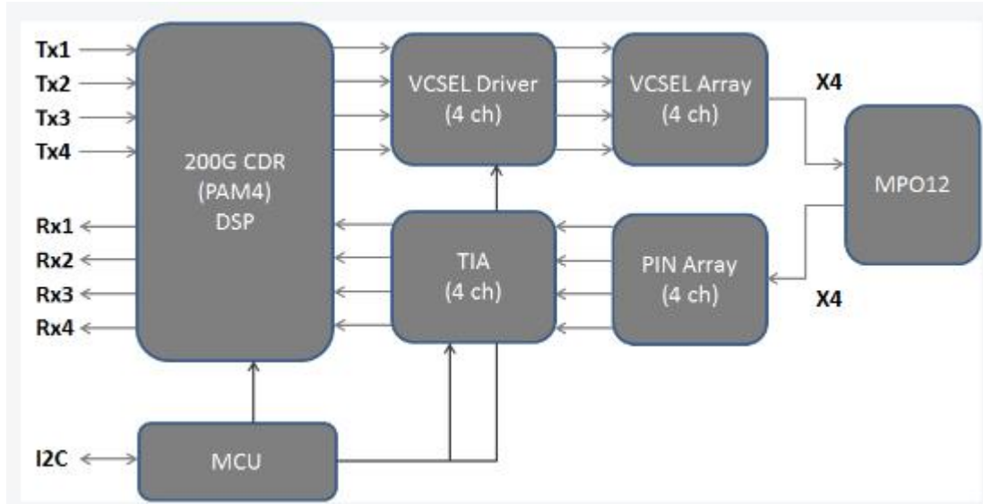
Figure 1. Module Block Diagram (200G End)
