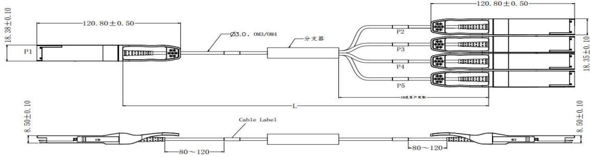
Figure 12. Mechanical Specifications
