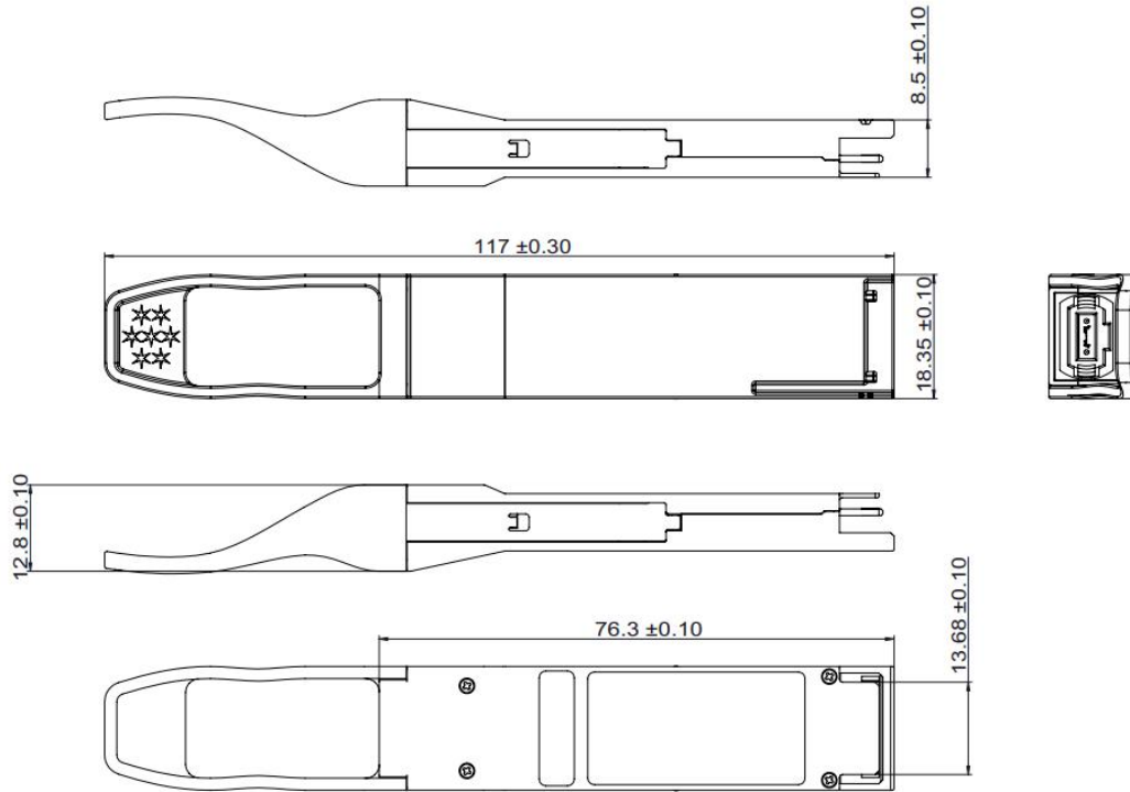
Figure 12. Mechanical Specifications
