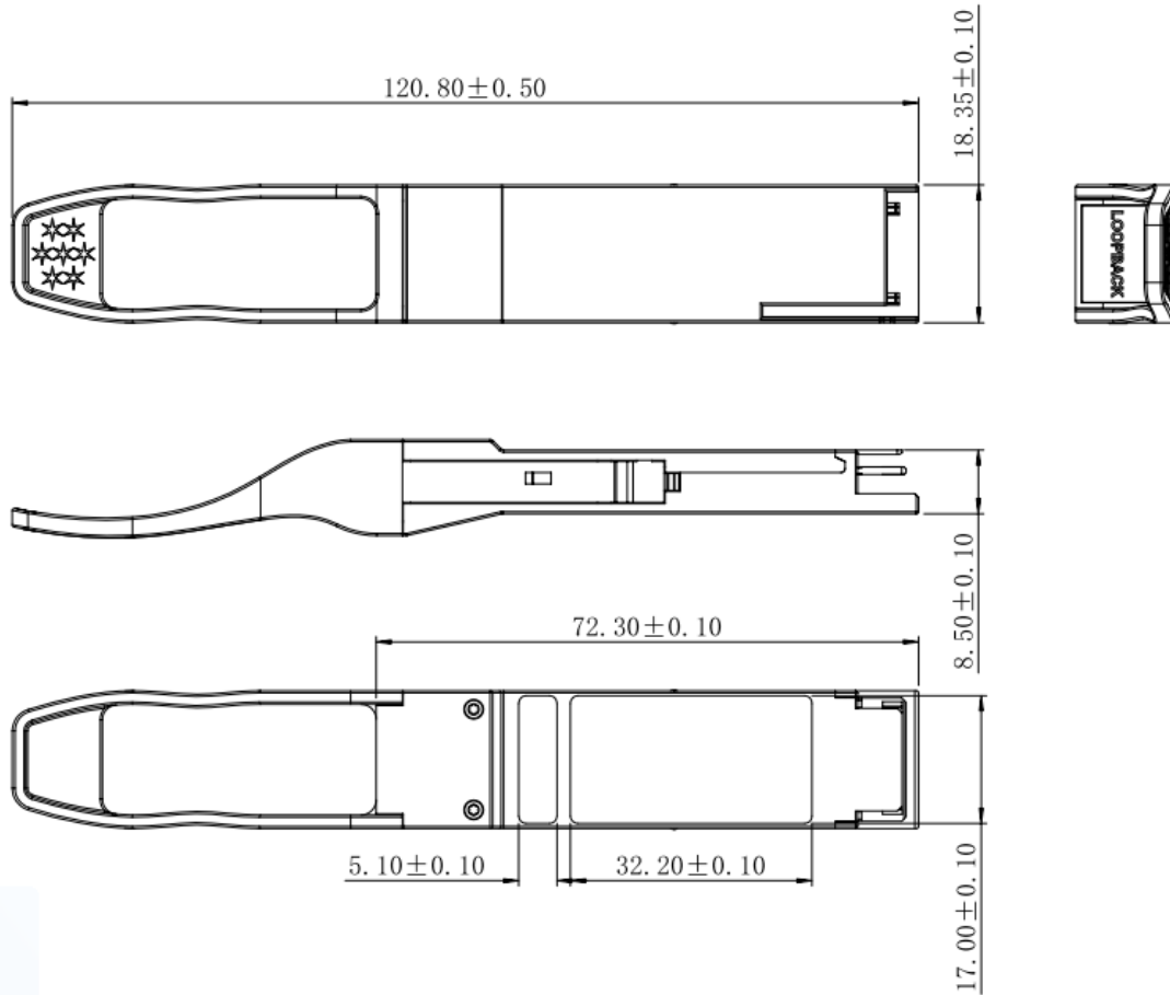
Figure 12. Mechanical Specifications
