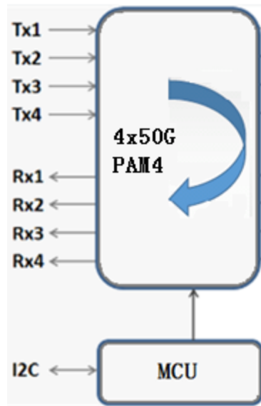
Figure 1. Module Block Diagram
