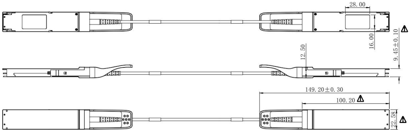
Figure5. Mechanical Specifications
