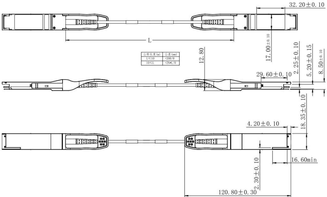
Figure5. Mechanical Specifications
