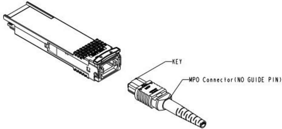
Figure10. Mechanical Specifications
