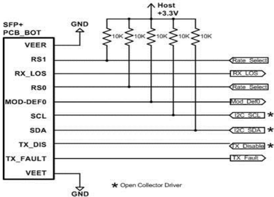
Figure 3.Recommended Interface Circuit
