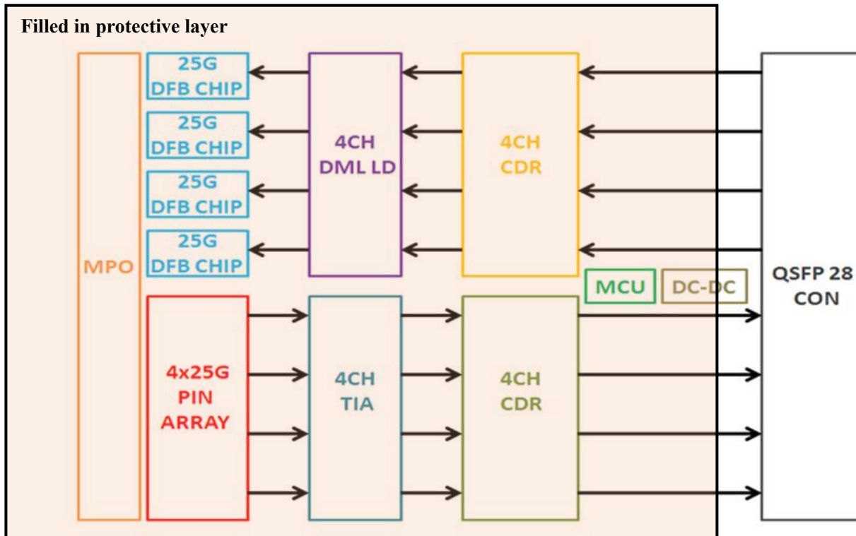
Figure1.Module Block Diagram
