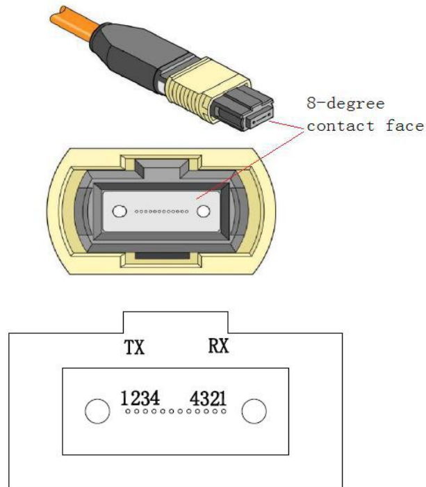
Figure10.Mechanical Specifications
