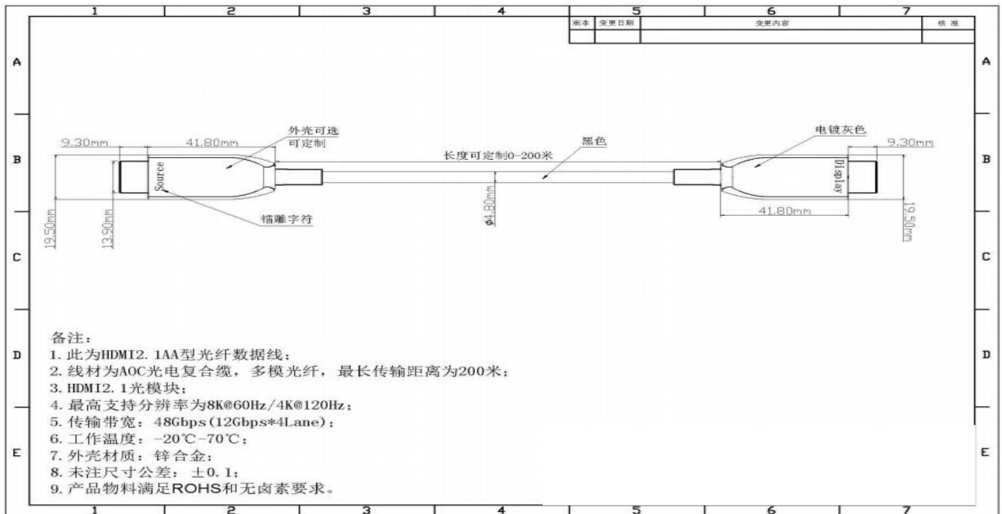
Figure 3. Mechanical Specifications
