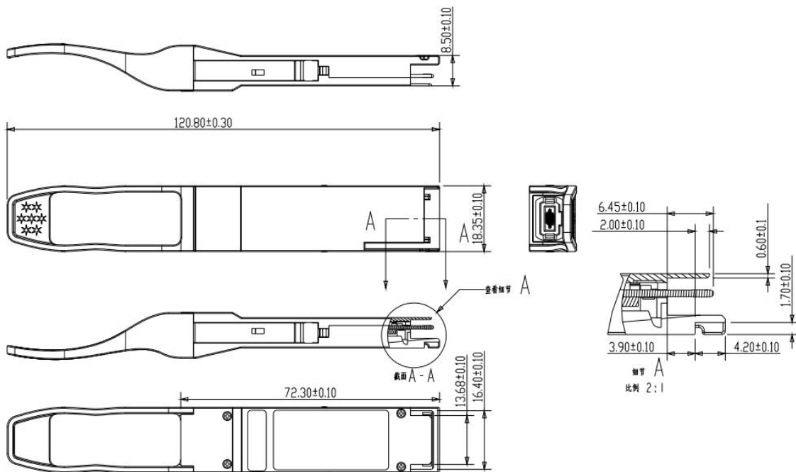
Figure 14. Mechanical Specifications
